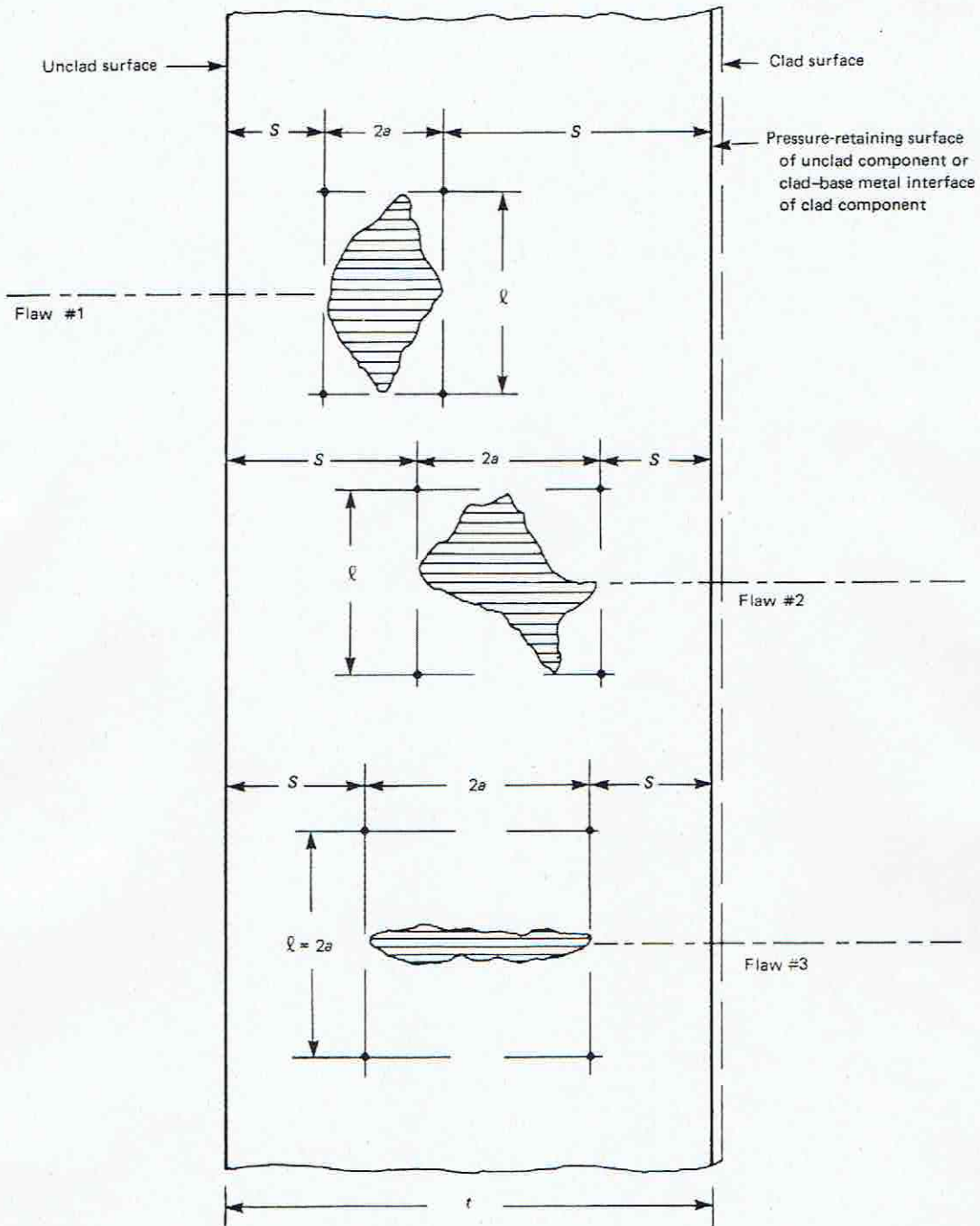
Figure IWA-3320-1 Subsurface Planar Flaws Oriented in Plane Normal to Pressure-Retaining Surface Illustrative Flaw Configurations and Determination of Dimensions 2a and l Where S/ls \geq 0.4a (1 in. = 25 mm)
